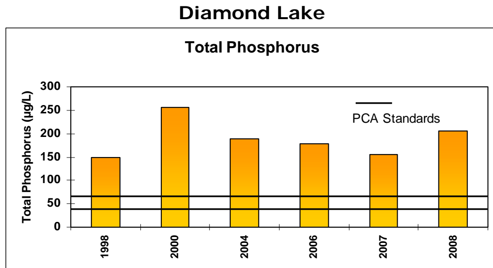
Figure 7 Diamond Lake annual changes in total phosphorus data. Values are the growing season average from May through September.
