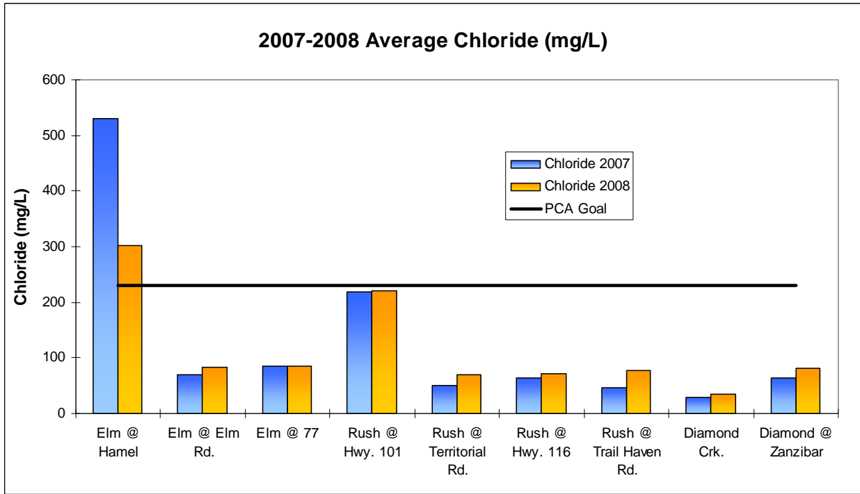
Figure 4 Average chloride (mg/L) for July-November 2007 and April-November 2008.
