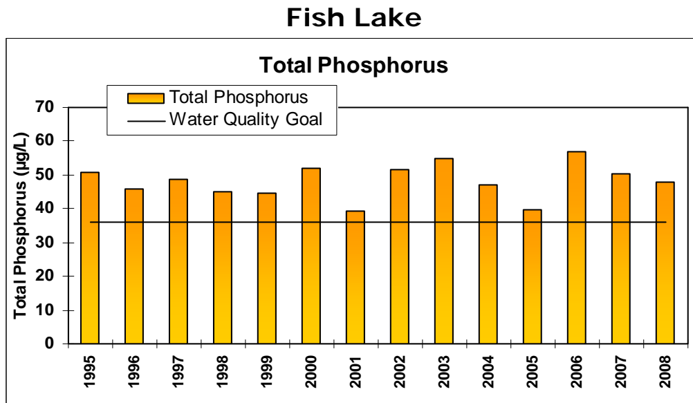
Figure 6 Fish Lake annual changes in total phosphorus data for 1995-2008. Values are the growing season average from May through September.
