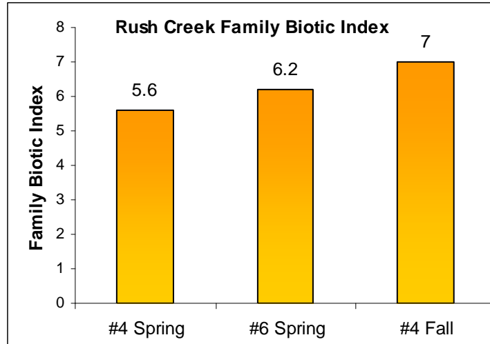
Figure 12 Family Biotic Index ratings for the two sites on Rush Creek in 2007.
