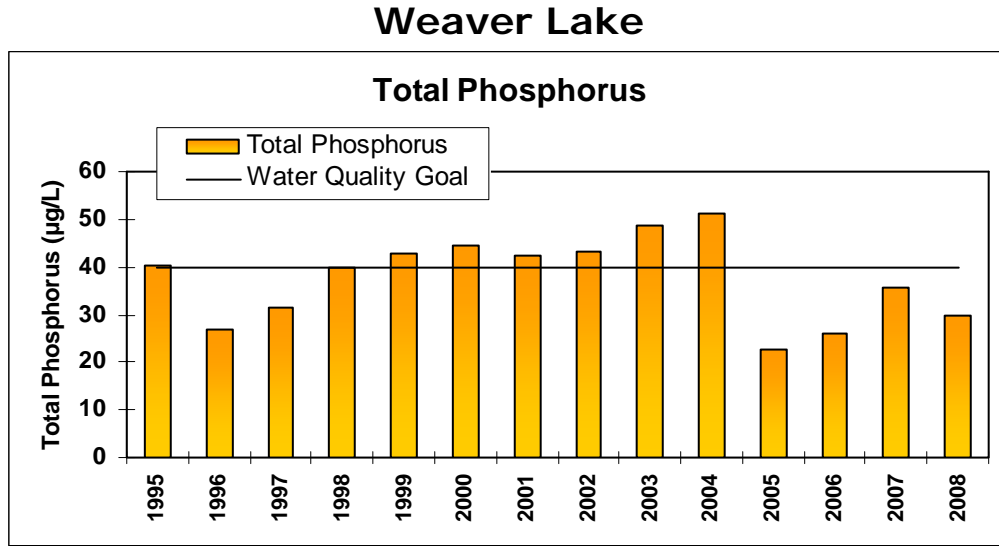
Figure 8 Weaver Lake annual changes in total phosphorus data for 1995-2008. Values are the growing season average from May through September.
