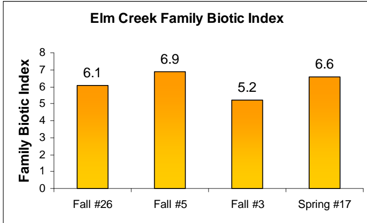
Figure 10 Family Biotic Index ratings for the four sites on Elm Creek in 2007.
